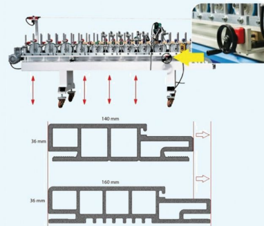
TEK TARAFLI AÇILIR KAPANIR KOLAY AYAR SİSTEMİ SINGLE SIDED ADJUSTMENT SYSTEM
